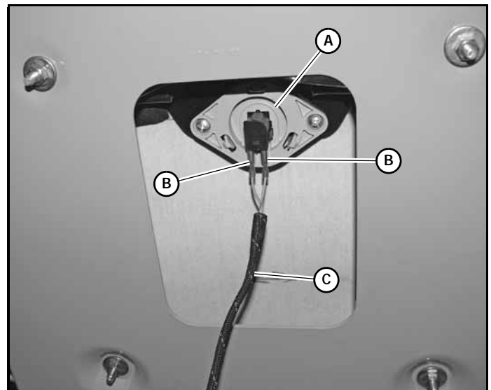
A. Seat switch B. Female spades
